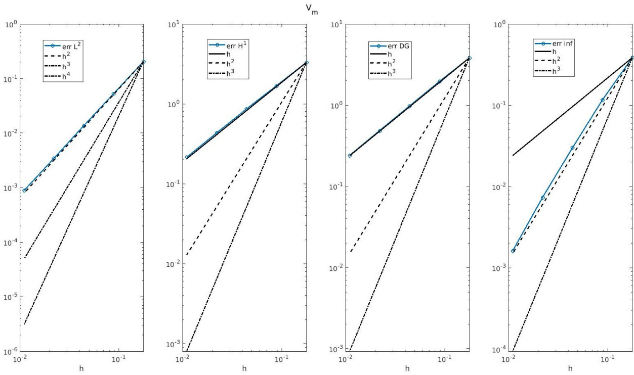
(a) V_m : Semi-implicit method with p = 1 Dubiner basis
