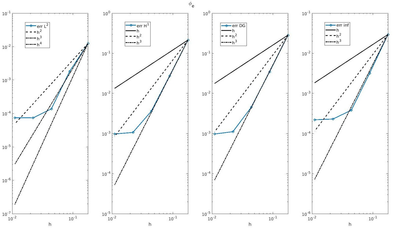
(b) Extracellular potential ( \phi_e ) with p = 3 Lagrangian hat functions
