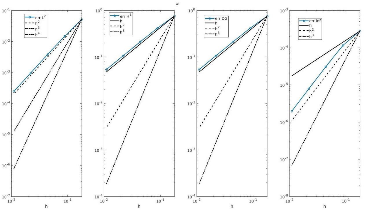
(b) Gating variable ( w ) with p = 1 Lagrangian hat functions
