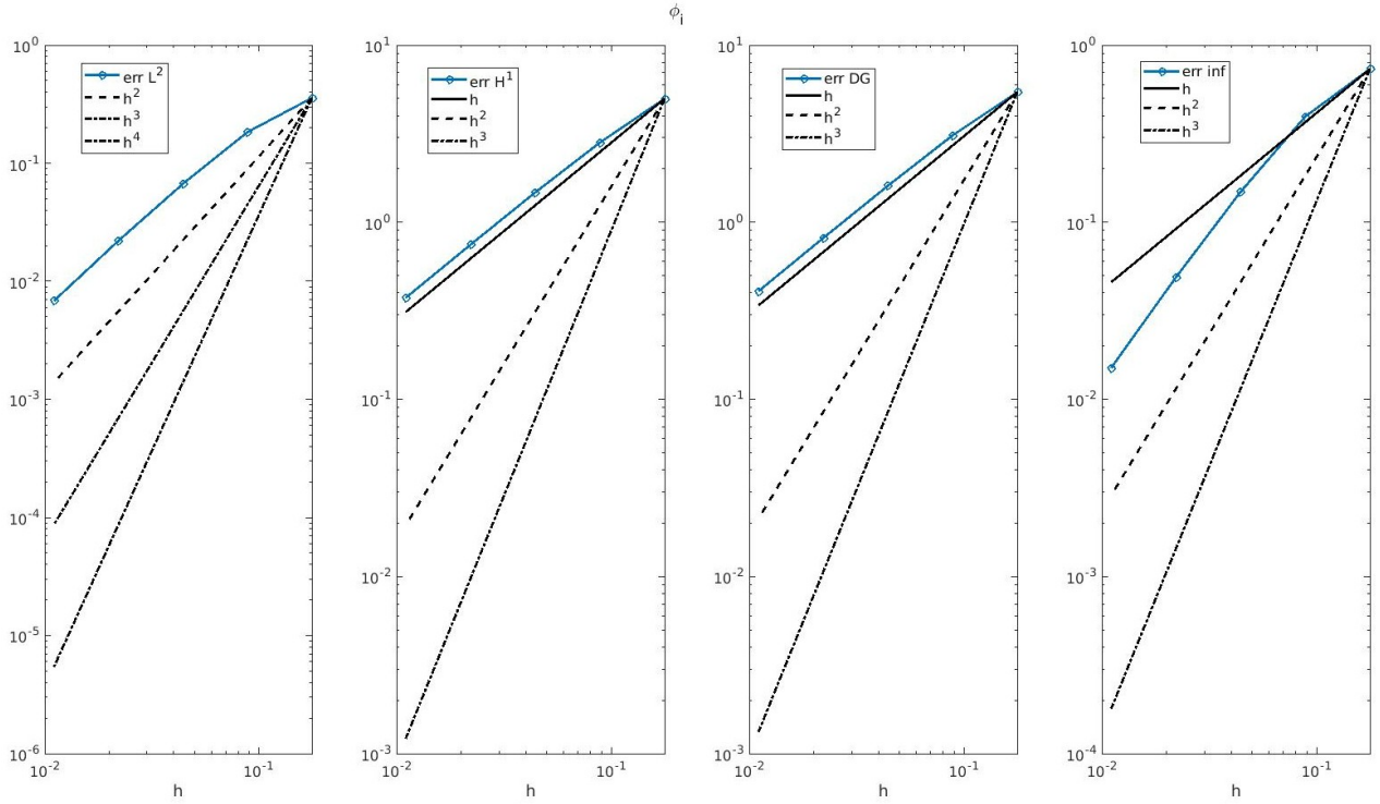
(b) Intracellular potential ( \phi_i ) with p = 1 Lagrangian hat functions
