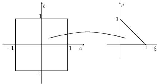
Figure 3: Transformation between the reference square ( \hat{Q} ) to the reference triangle ( \hat{K} )
