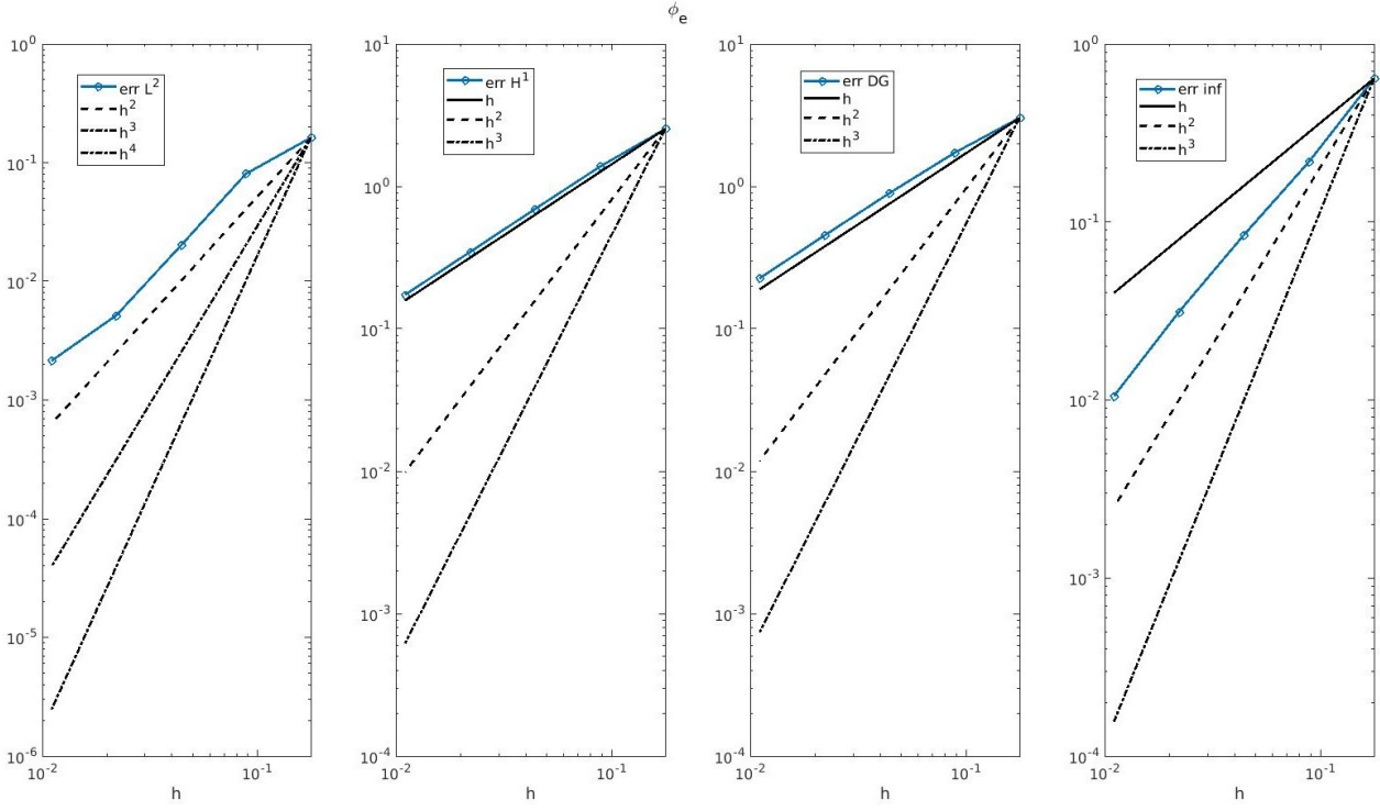
(a) \phi_e : imposing the first coefficient with p = 1 Dubiner basis
