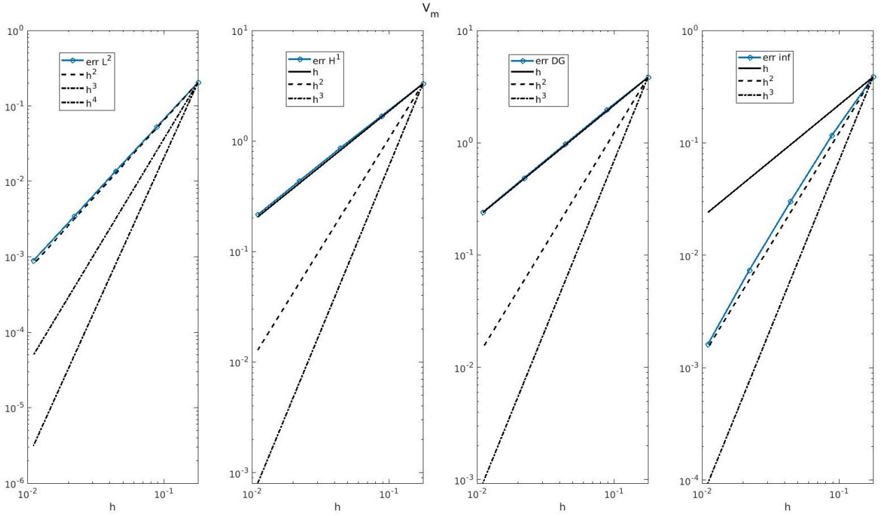
(a) Trans-membrane potential ( V_m ) with p = 1 Dubiner basis
