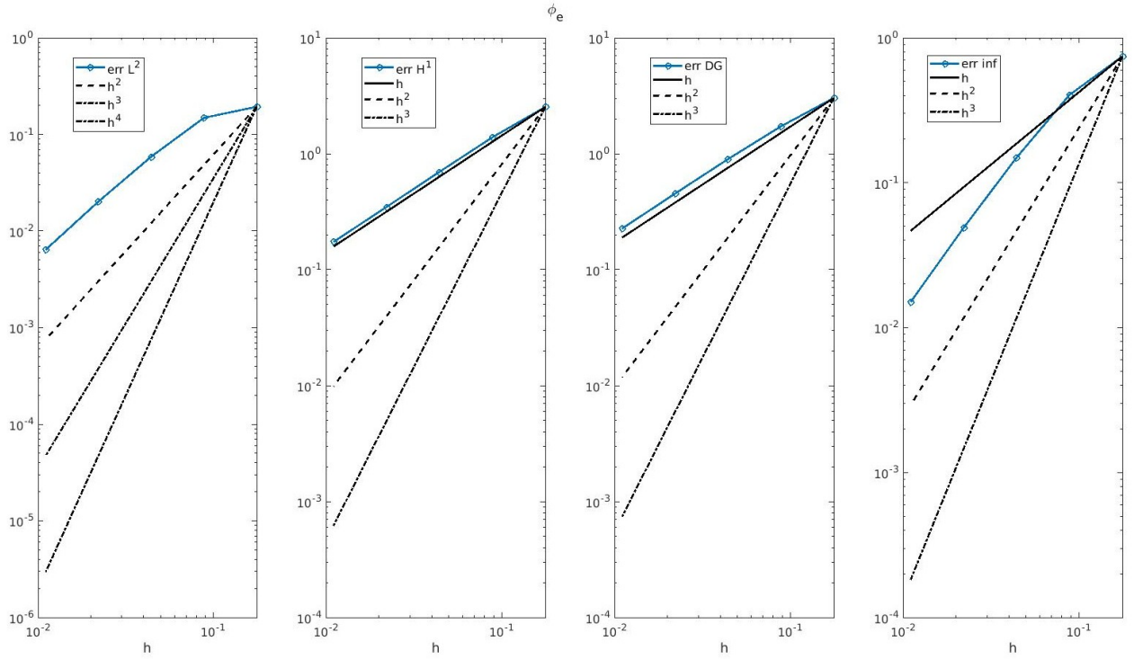
(b) Extracellular potential ( \phi_e ) with p = 1 Lagrangian hat functions
