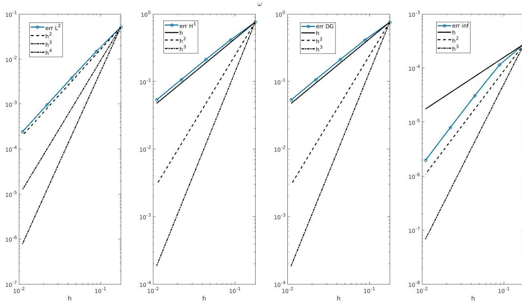
(a) Gating variable ( w ) with p = 1 Dubiner basis
