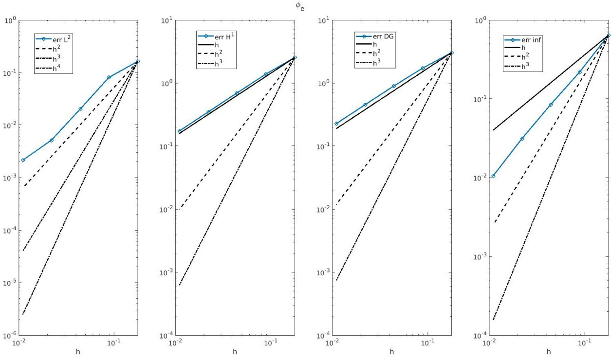
(a) \phi_e : Semi-implicit method with p = 1 Dubiner basis
