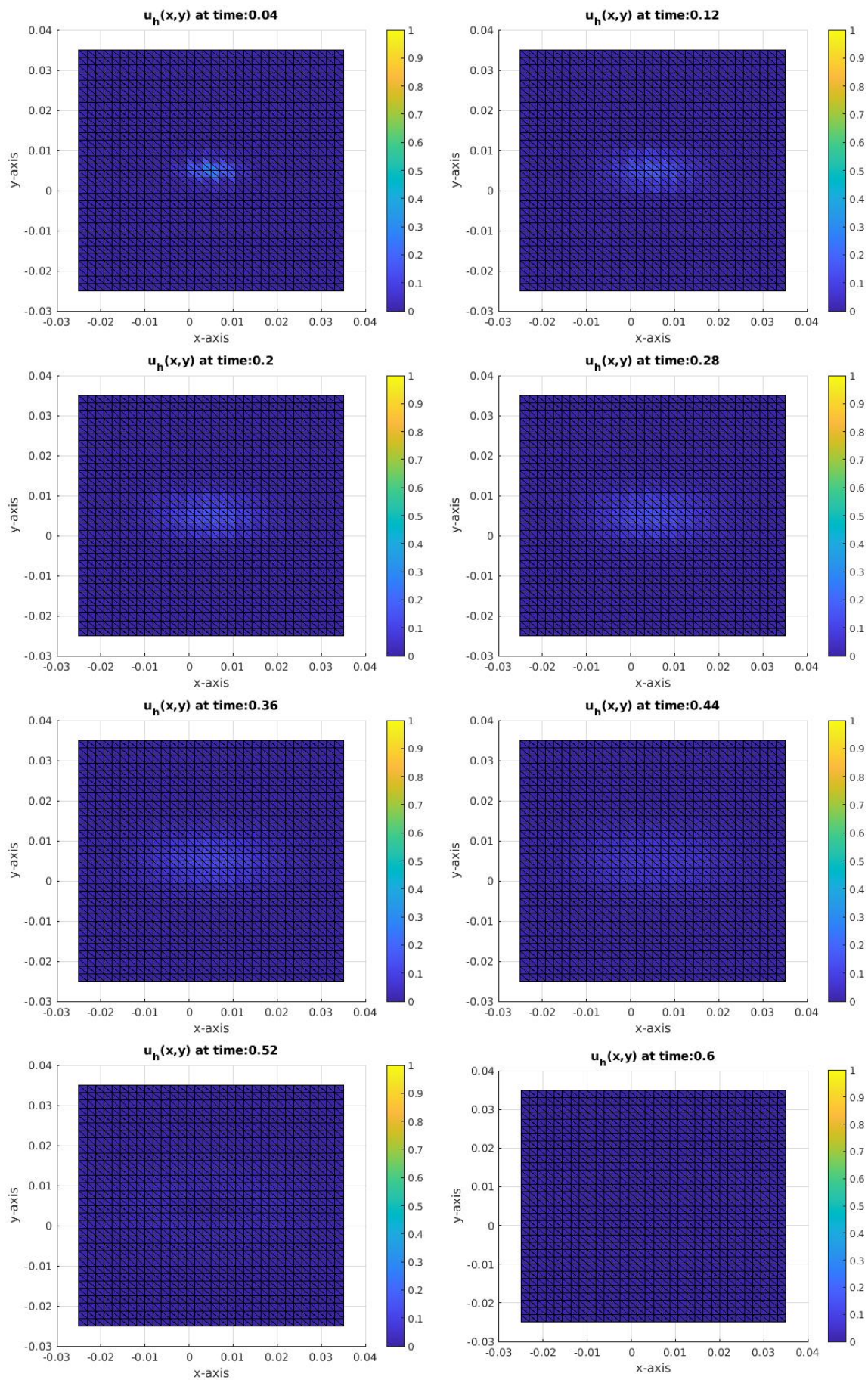
Figure 27: Test-case 2, computed snapshots for underflow case ( I = 15000 \cdot 10^3 Am^{-3} )
