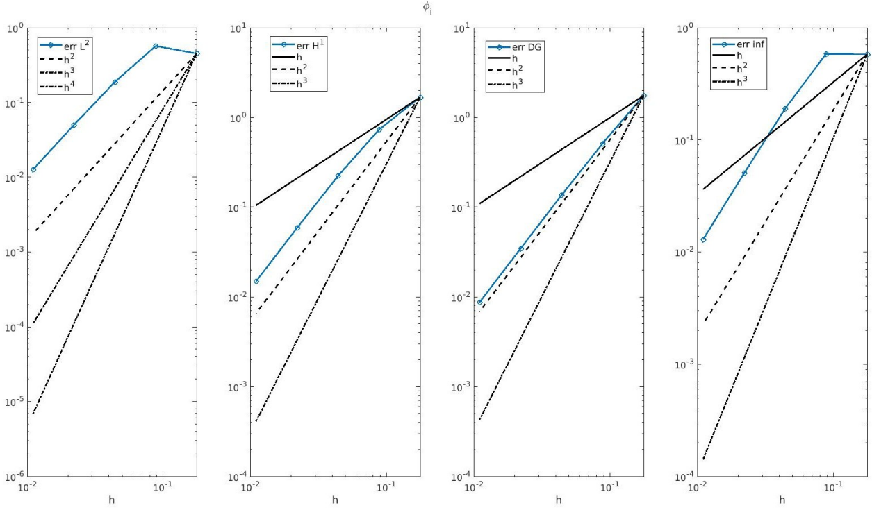
(a) Intracellular potential ( \phi_i ) with p = 2 Dubiner basis
