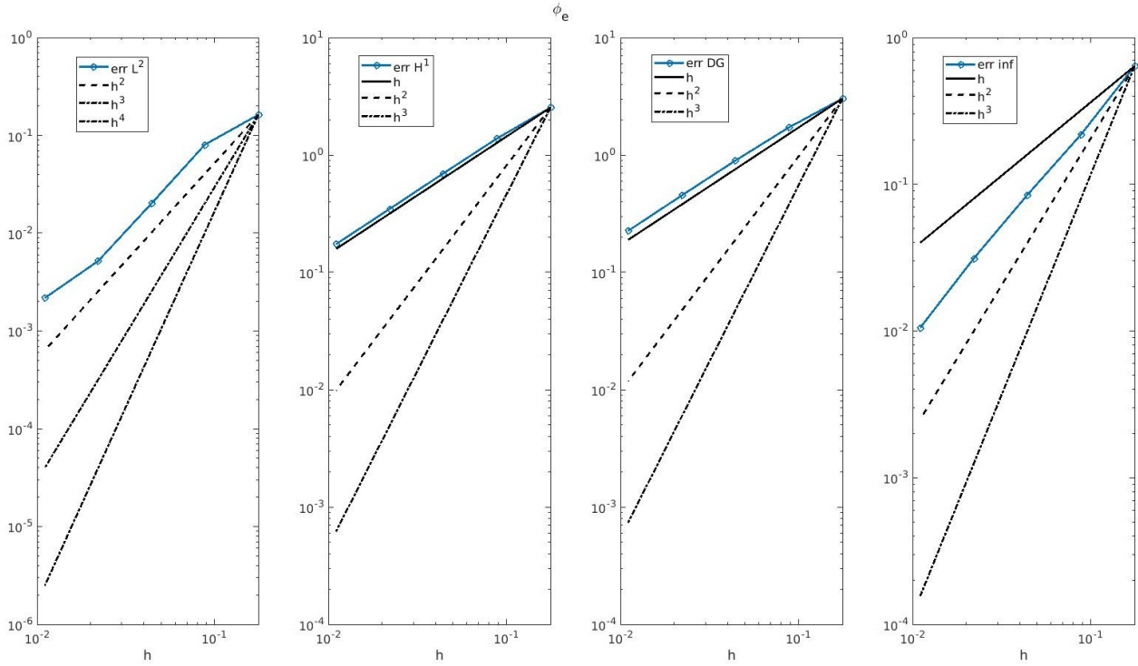
(b) \phi_e : Godunov operator-splitting method with p = 1 Dubiner basis
