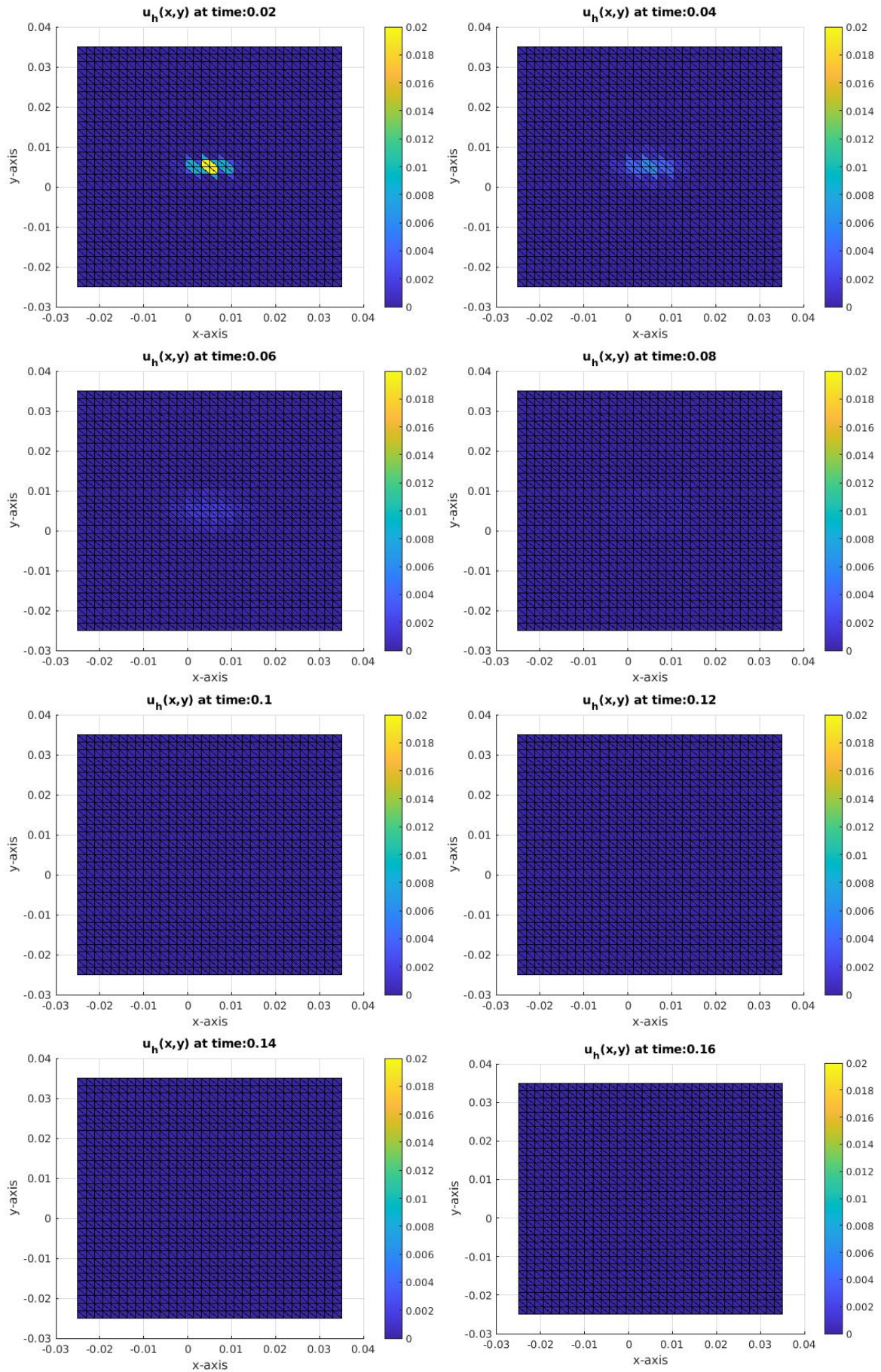
Figure 25: Test-case 1, computed snapshots for underflow case ( I = 500 \cdot 10^3 Am^{-3} )
