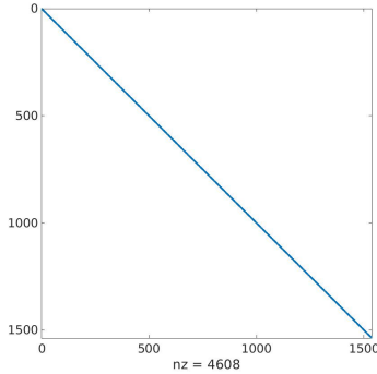
Figure 4: Non-zero elements in the mass matrix when adopting Dubiner basis
