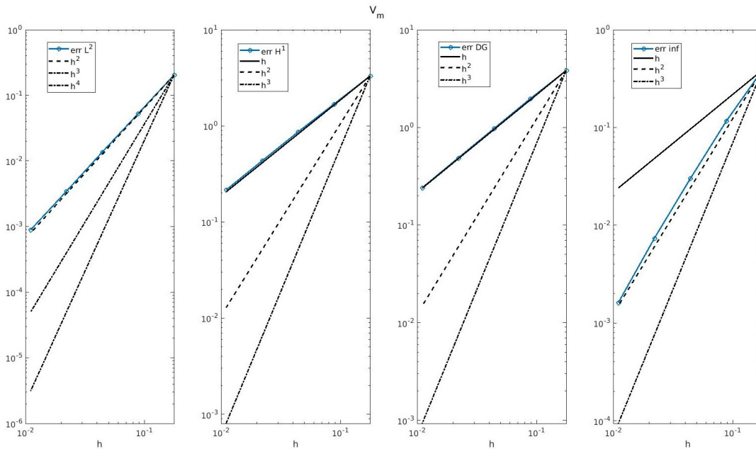
(b) Trans-membrane potential ( V_m ) with p = 1 Lagrangian hat functions
