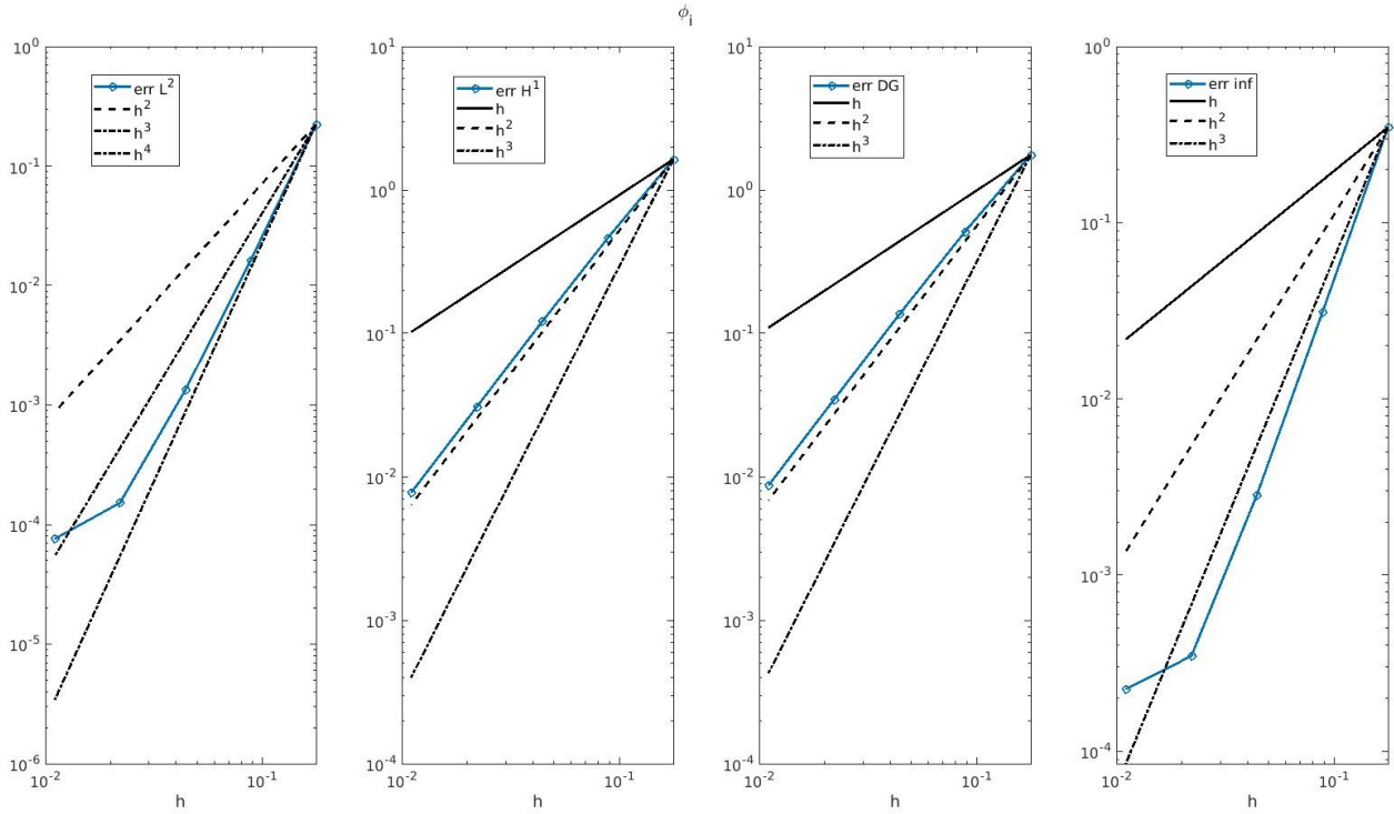
(b) Intracellular potential ( \phi_i ) with p = 2 Lagrangian hat functions
