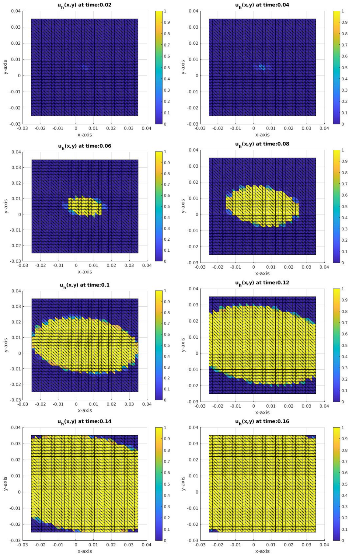
Figure 26: Test-case 1, computed snapshots for overflow case ( I = 700 \cdot 10^3 Am^{-3} )
