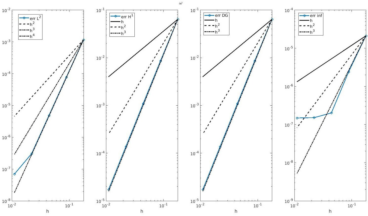
(a) Gating variable ( w ) with p = 3 Dubiner basis
