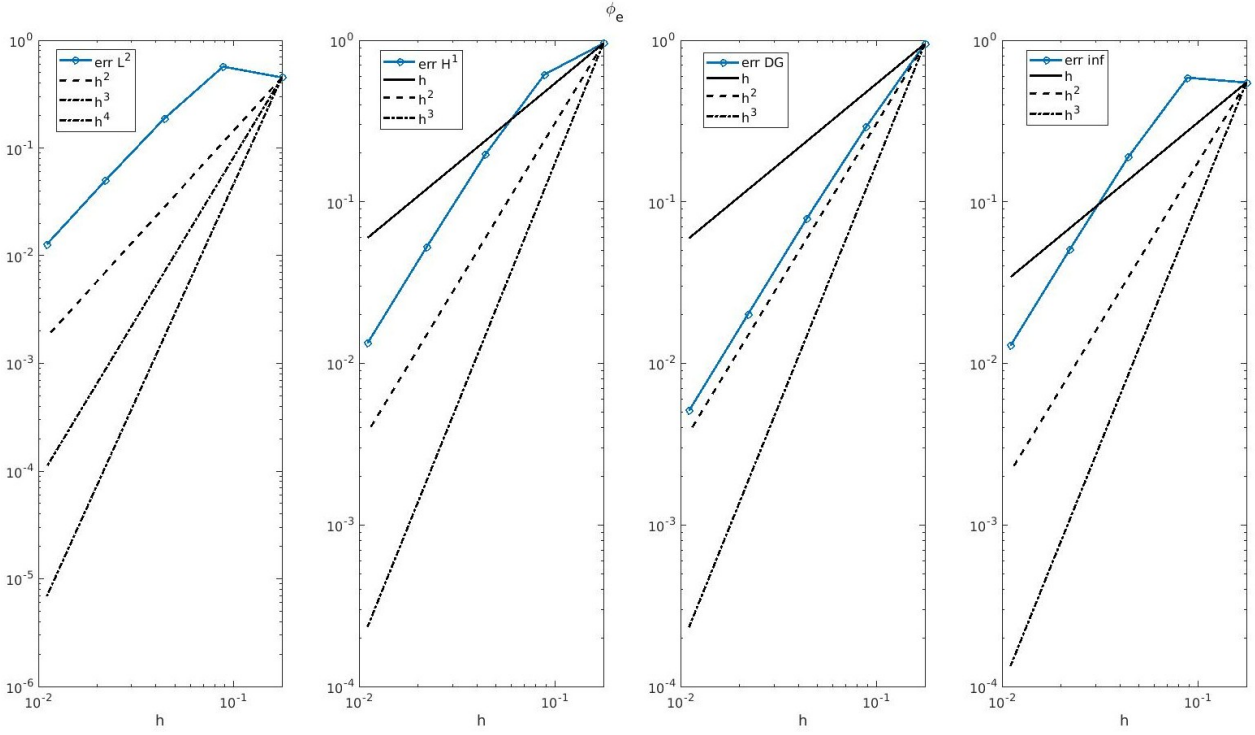
(a) Extracellular potential ( \phi_e ) with p = 2 Dubiner basis
