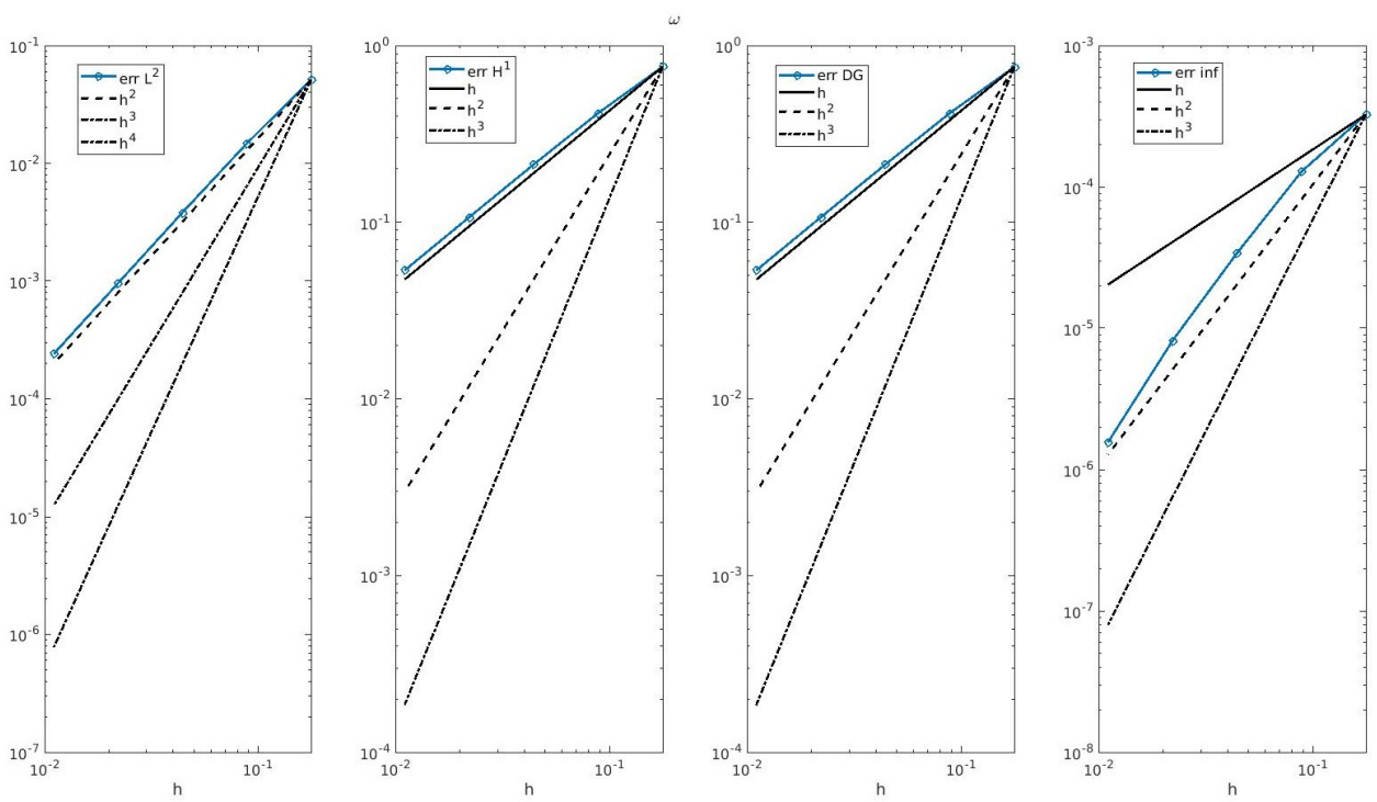
(c) w : Quasi-implicit operator-splitting method with p = 1 Dubiner basis
