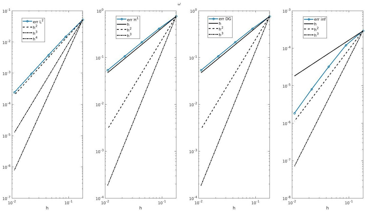
(b) w : Godunov operator-splitting method with p = 1 Dubiner basis
