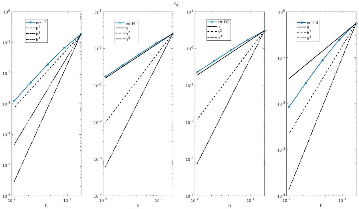
(b) \phi_e : imposing the zero mean with p = 1 Dubiner basis
