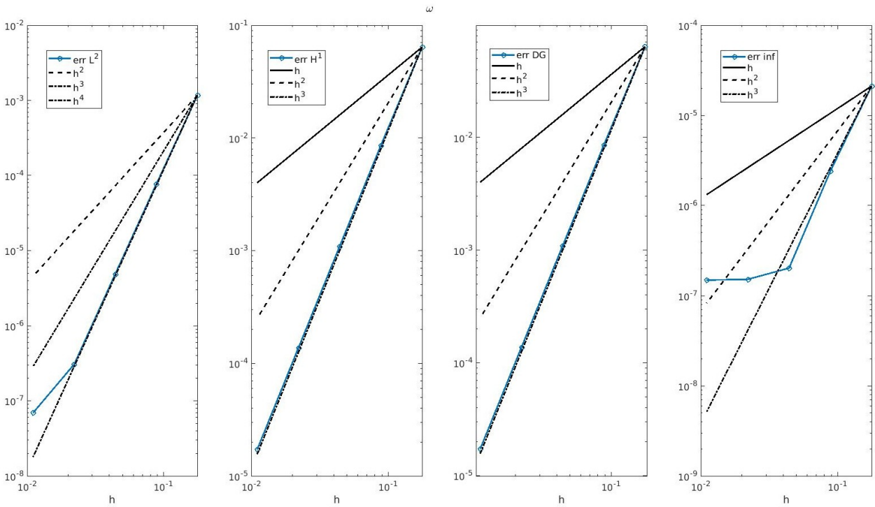
(b) Gating variable ( w ) with p = 3 Lagrangian hat functions
