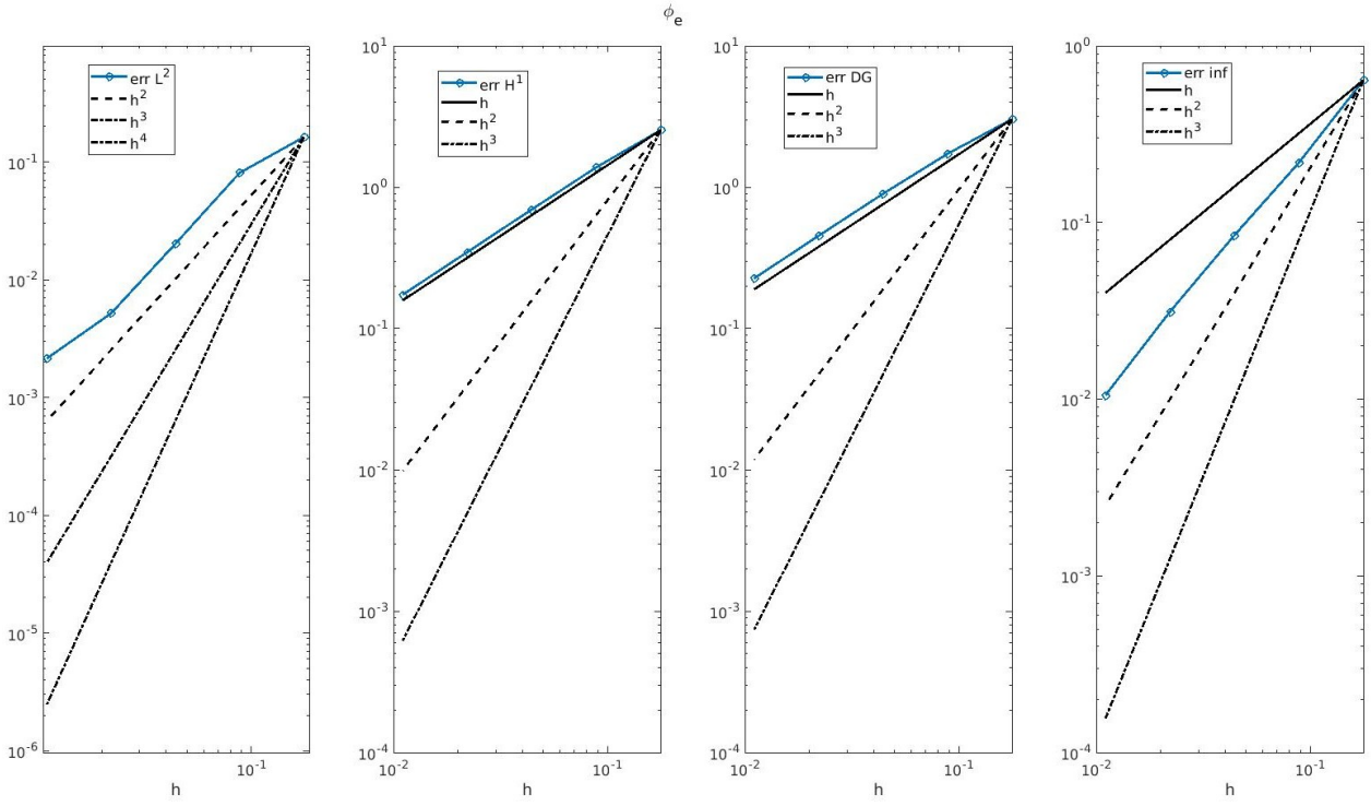
(c) \phi_e : Quasi-implicit operator-splitting method with p = 1 Dubiner basis
