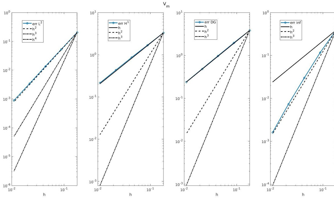
(a) Trans-membrane potential ( V_m ) with p = 1 Dubiner basis
