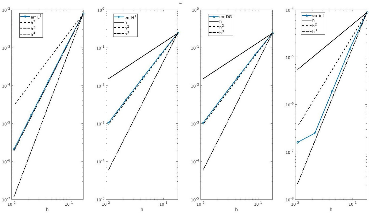
(b) Gating variable ( w ) with p = 2 Lagrangian hat functions
