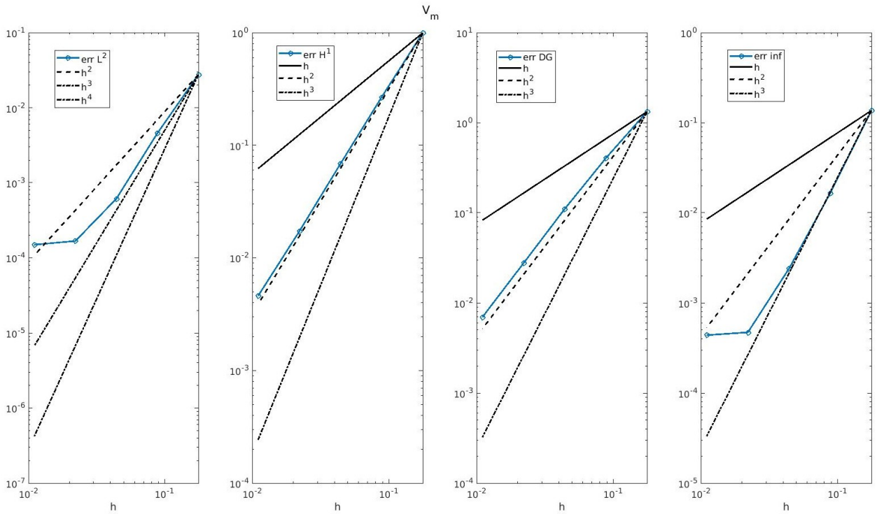
(b) Trans-membrane potential ( V_m ) with p = 2 Lagrangian hat functions
