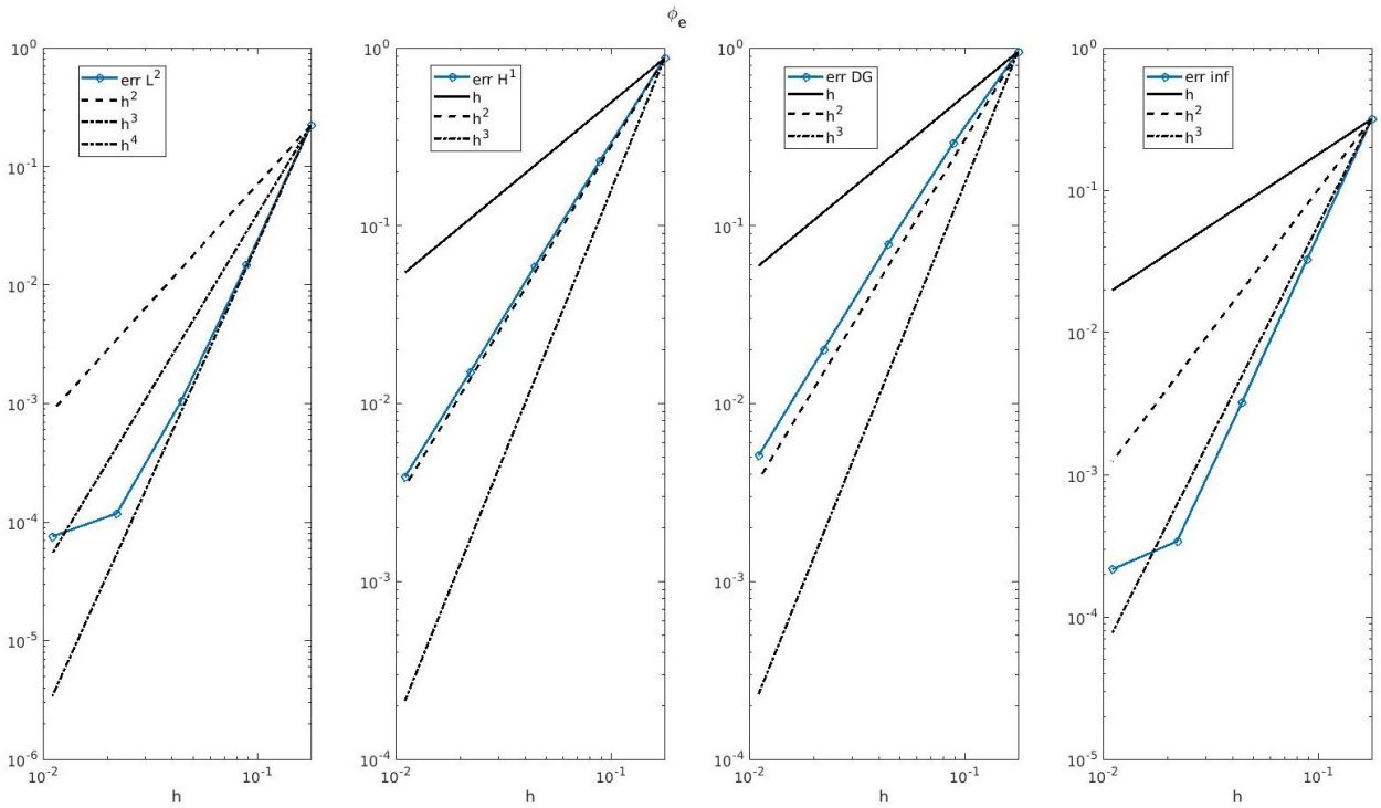
(b) Extracellular potential ( \phi_e ) with p = 2 Lagrangian hat functions
