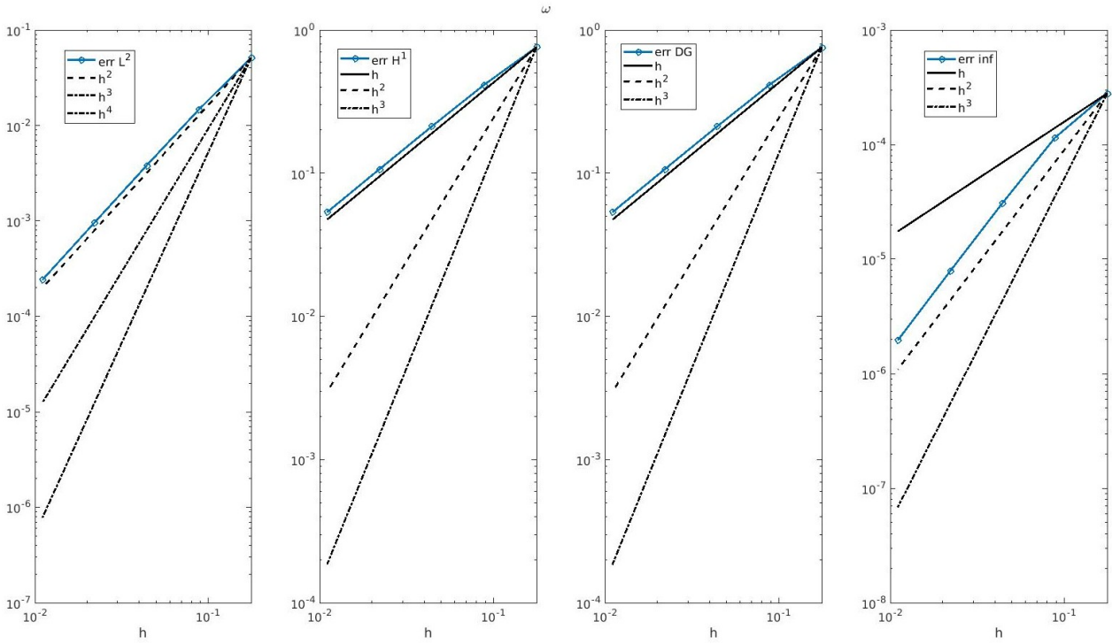
(a) w : Semi-implicit method with p = 1 Dubiner basis
