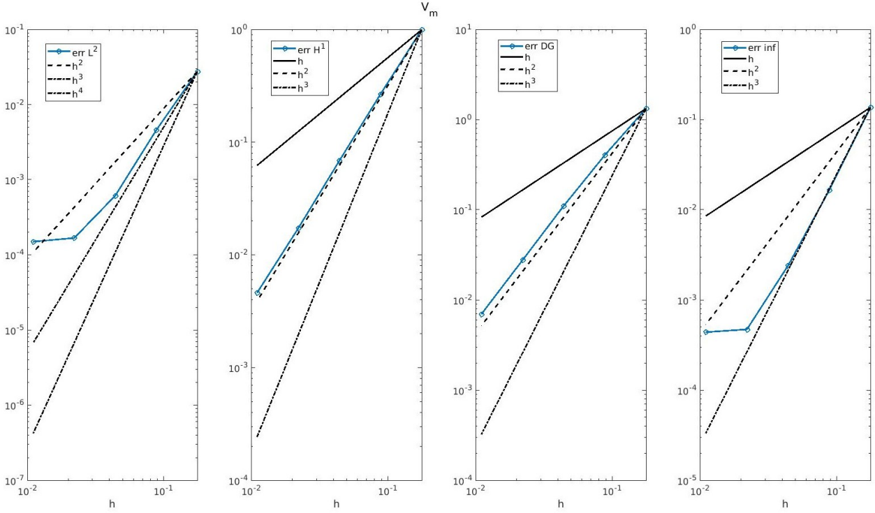
(a) Trans-membrane potential ( V_m ) with p = 2 Dubiner basis
