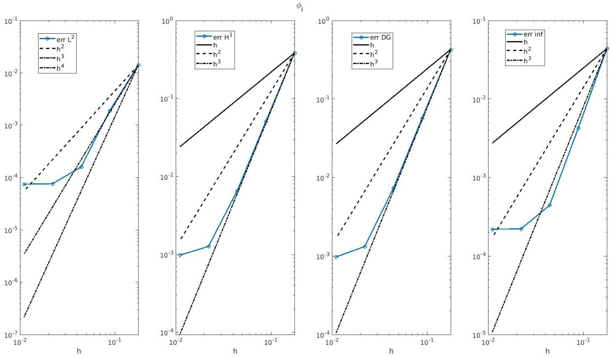
(b) Intracellular potential ( \phi_i ) with p = 3 Lagrangian hat functions
