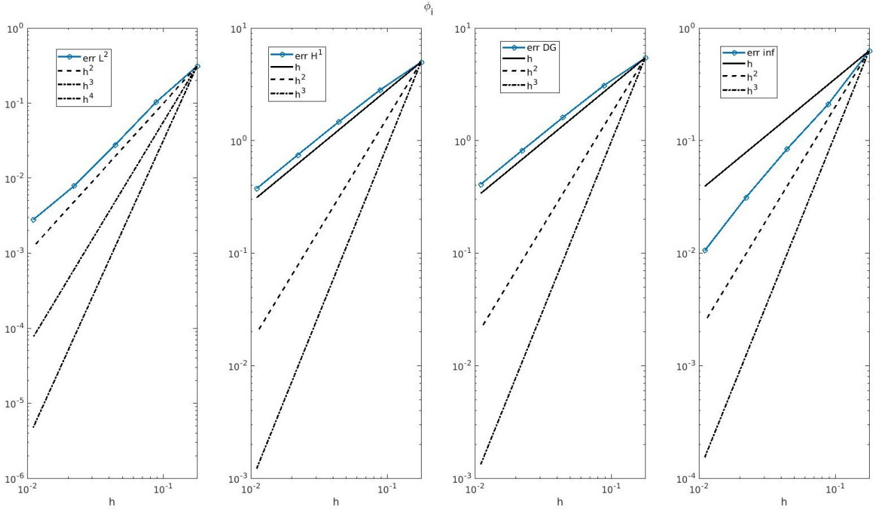
(a) Intracellular potential ( \phi_i ) with p = 1 Dubiner basis
