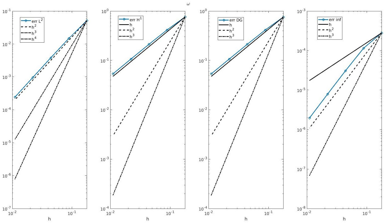
(b) w : imposing the zero mean with p = 1 Dubiner basis
