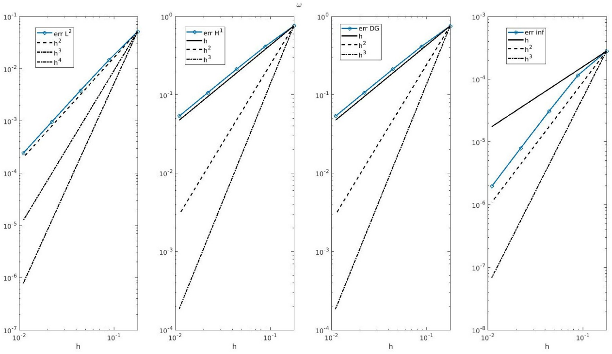
(a) w : imposing the first coefficient with p = 1 Dubiner basis
