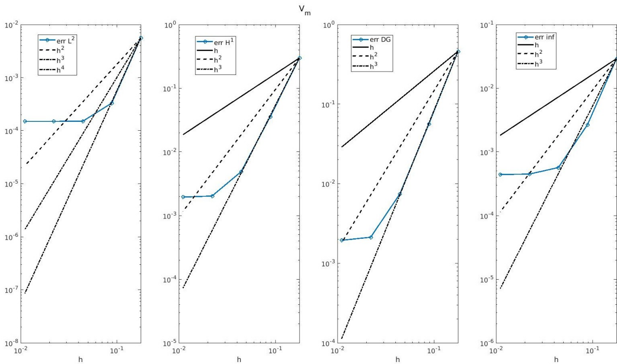
(b) Trans-membrane potential ( V_m ) with p = 3 Lagrangian hat functions
