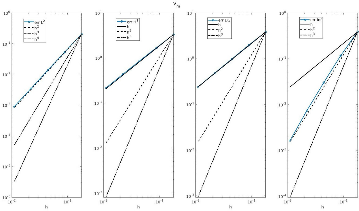
(c) V_m : Quasi-implicit operator-splitting method with p = 1 Dubiner basis
