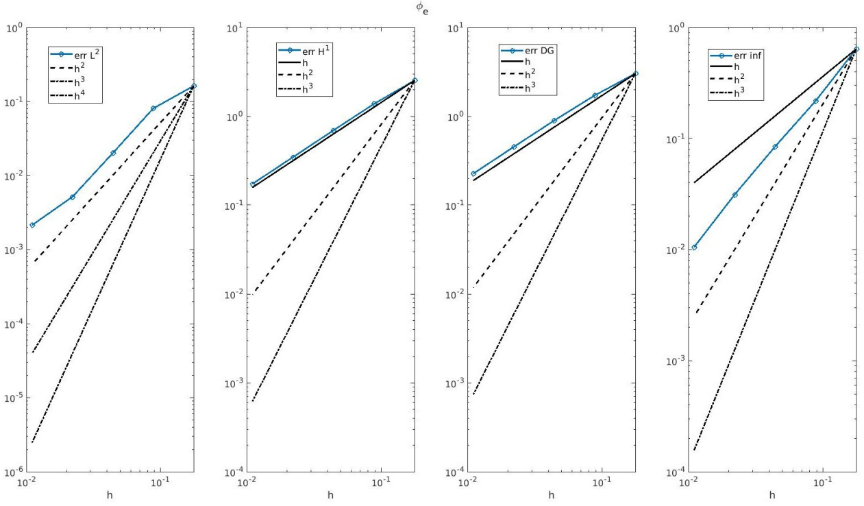
(a) Extracellular potential ( \phi_e ) with p = 1 Dubiner basis
