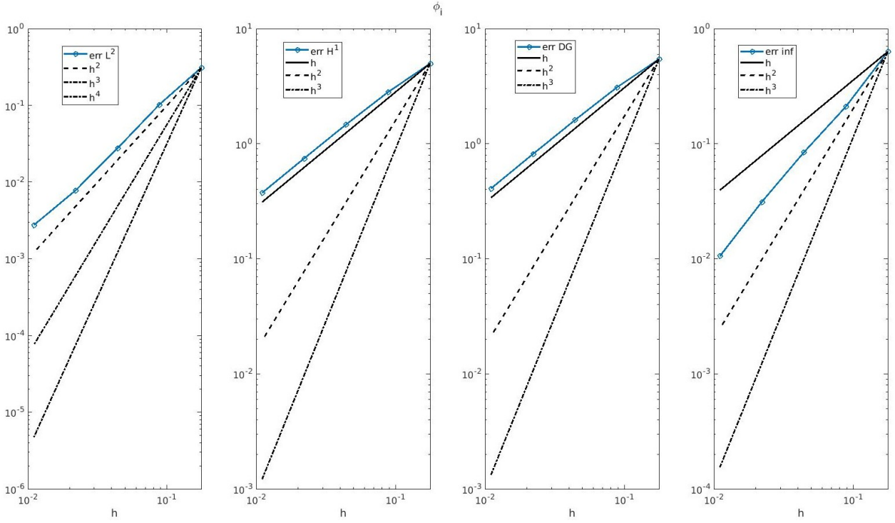
(b) \phi_i : Godunov operator-splitting method with p = 1 Dubiner basis
