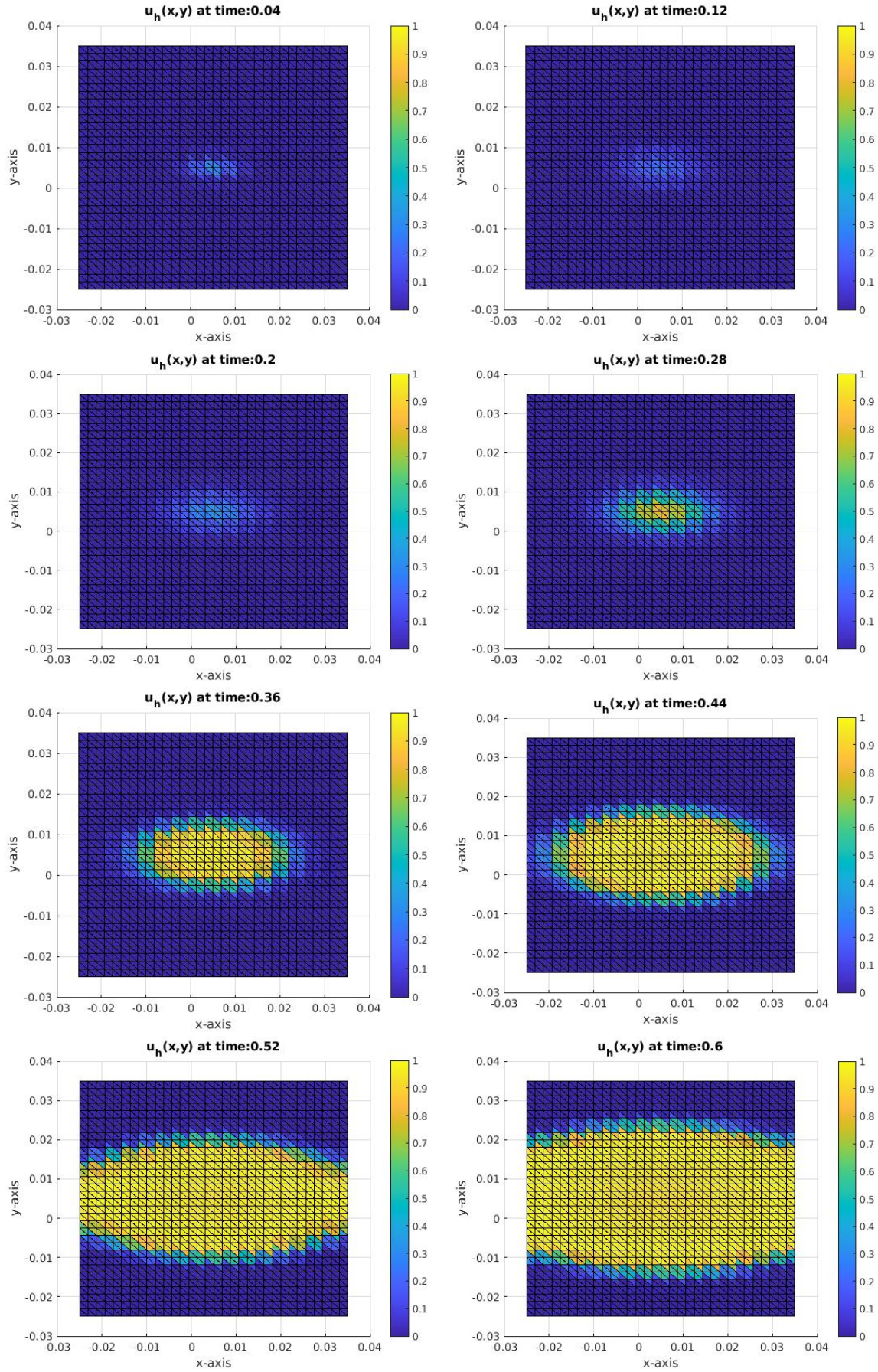
Figure 28: Test-case 2, computed snapshots for overflow case ( I = 20000 \cdot 10^3 Am^{-3} )
