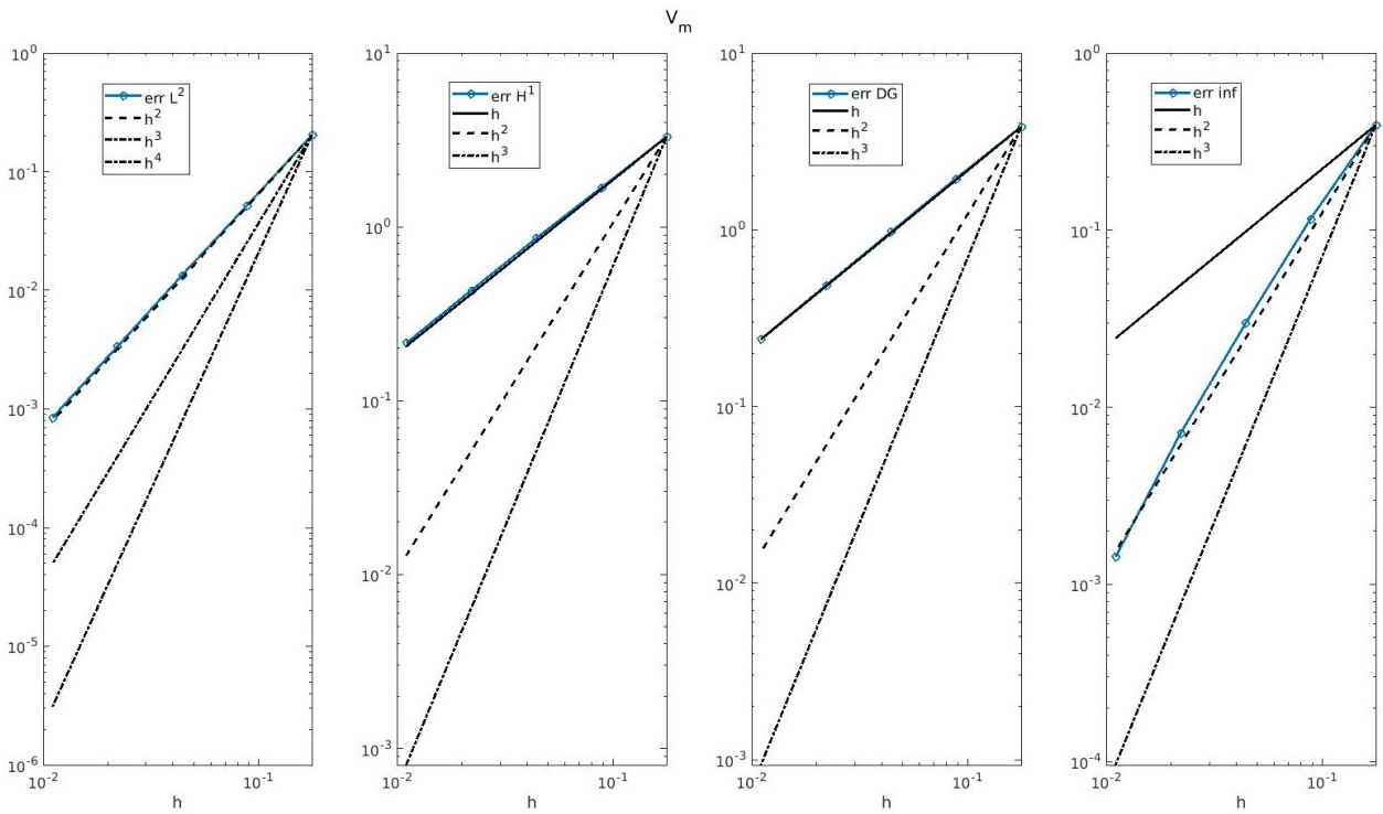
(b) V_m : Godunov operator-splitting method with p = 1 Dubiner basis
