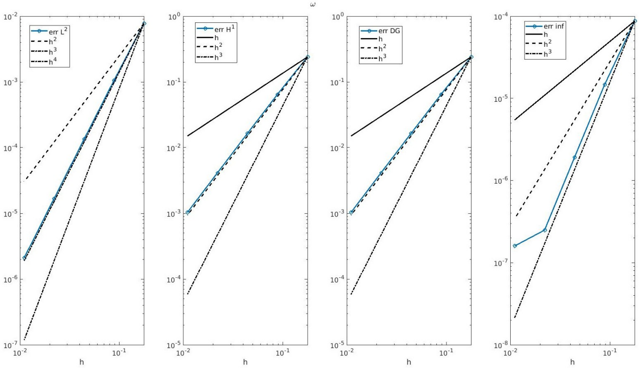
(a) Gating variable ( w ) with p = 2 Dubiner basis
