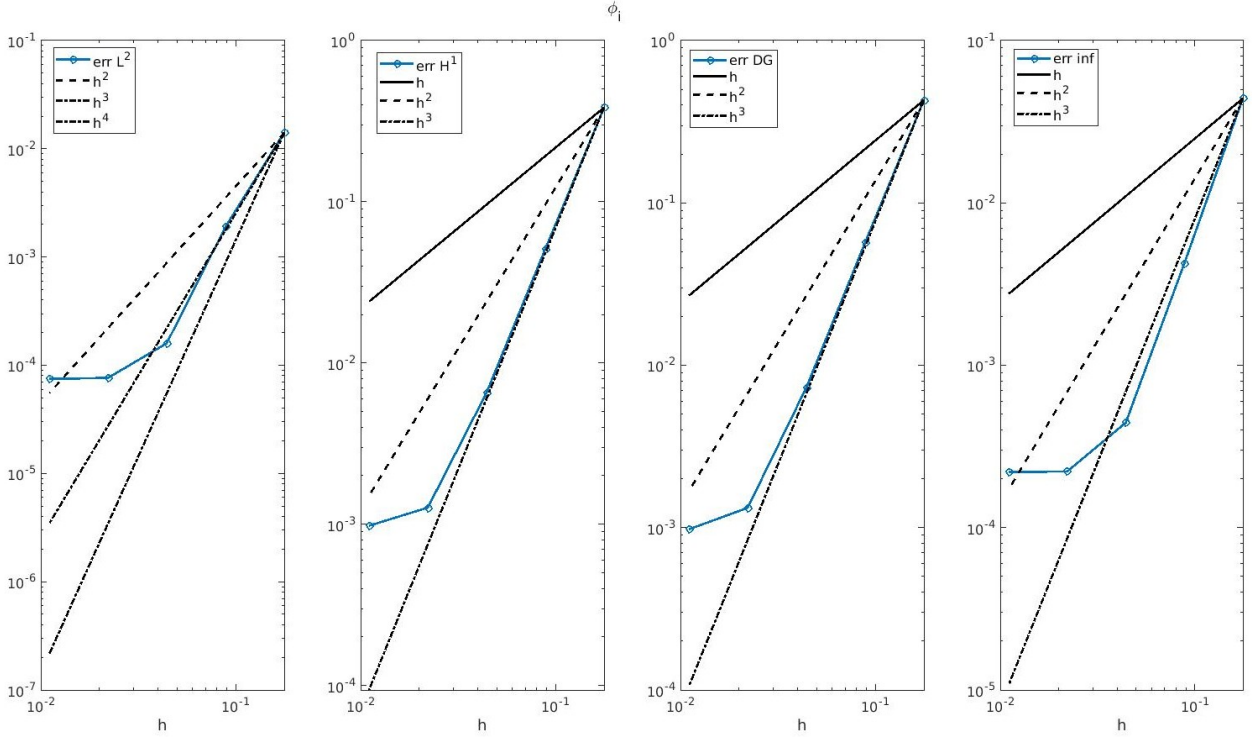
(a) Intracellular potential ( \phi_i ) with p = 3 Dubiner basis
