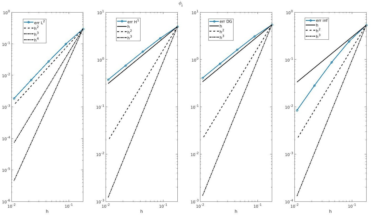
(b) \phi_i : imposing the zero mean with p = 1 Dubiner basis
