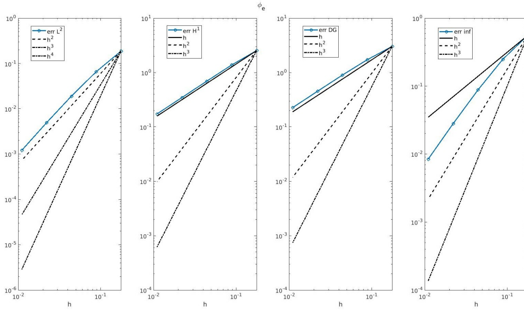
(b) Extracellular potential ( \phi_e ) with p = 1 Lagrangian hat functions
