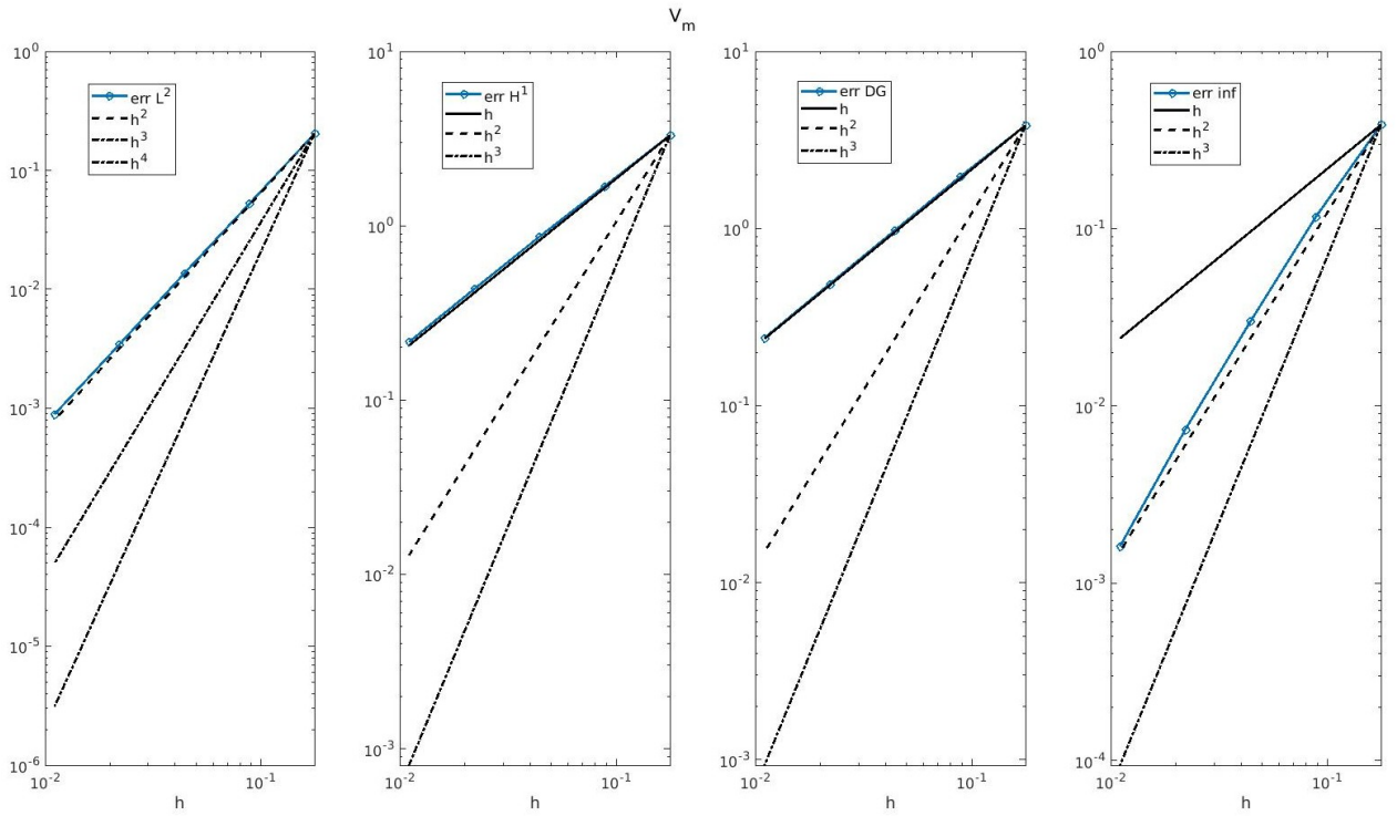
(b) V_m : imposing the zero mean with p = 1 Dubiner basis
