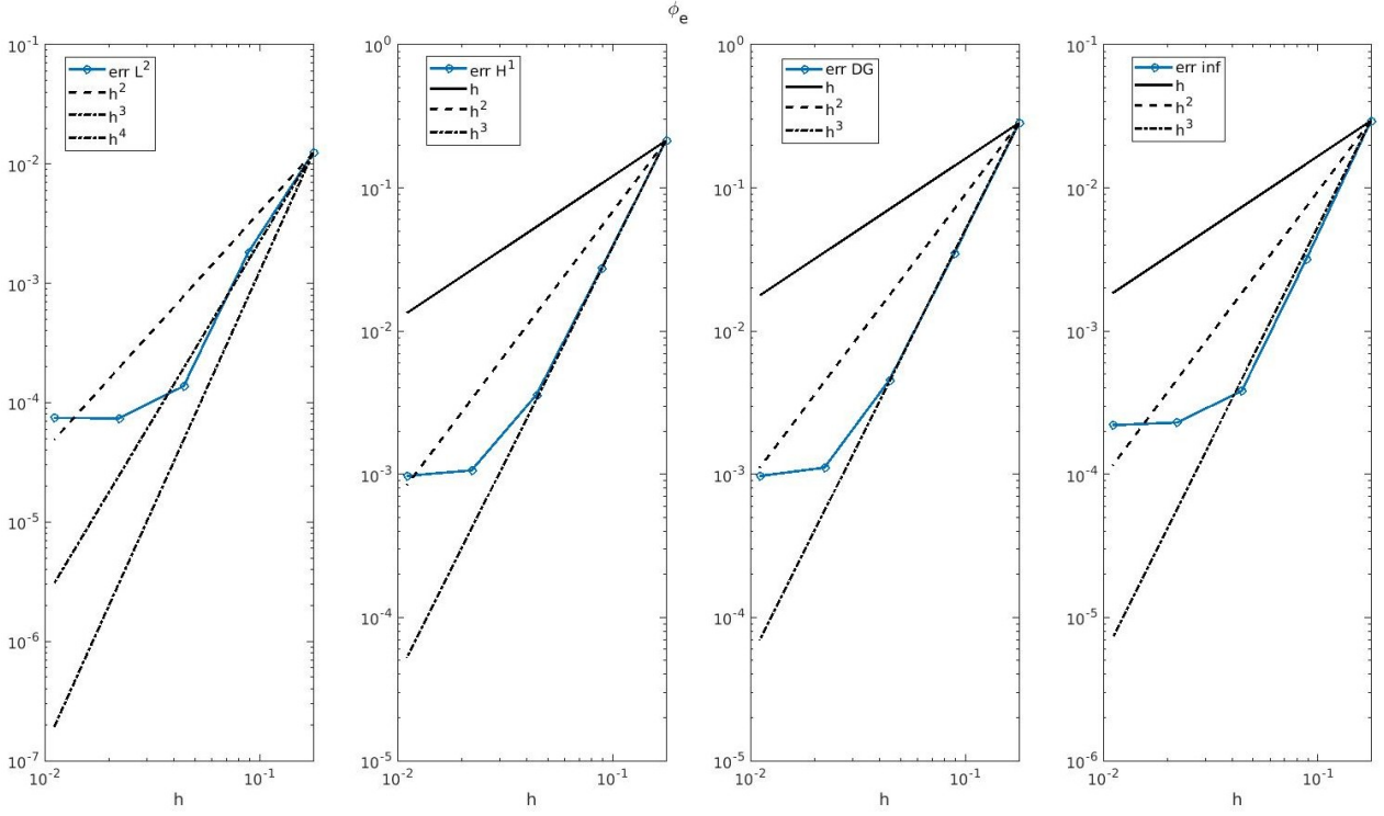
(a) Extracellular potential ( \phi_e ) with p = 3 Dubiner basis
