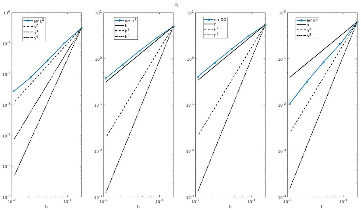
(c) \phi_i : Quasi-implicit operator-splitting method with p = 1 Dubiner basis
