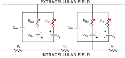
Figure 2: Simplified circuit to model the intracellular and extracellular potential dynamics
